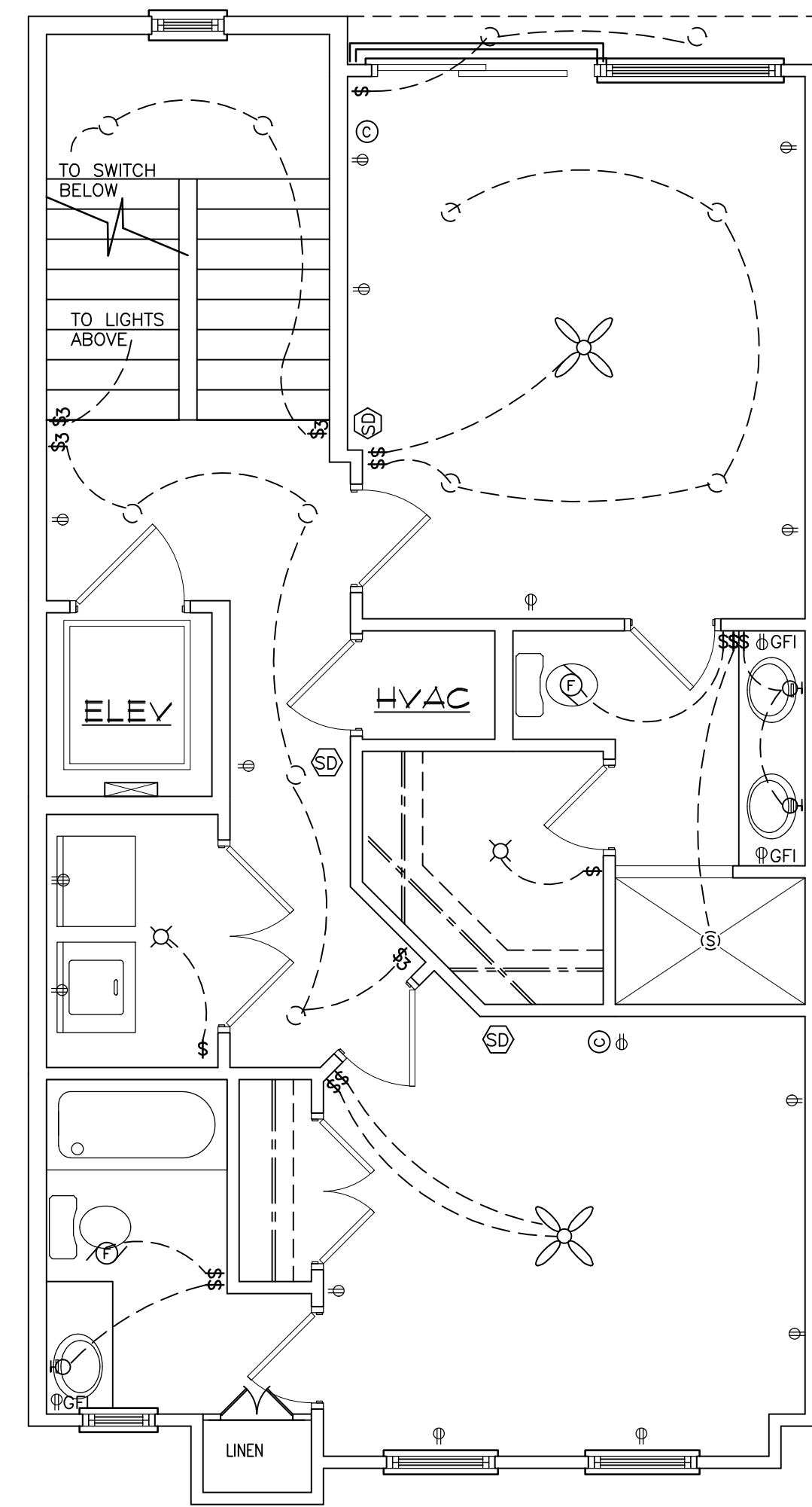
SECOND FLOOR PLAN 1/4"=1'-0"
