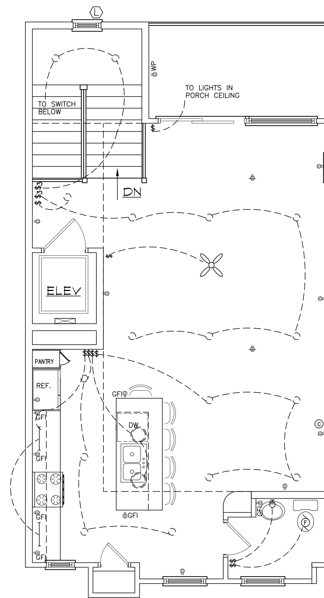
THIRD FLOOR PLAN 1/4"=1'-0"
